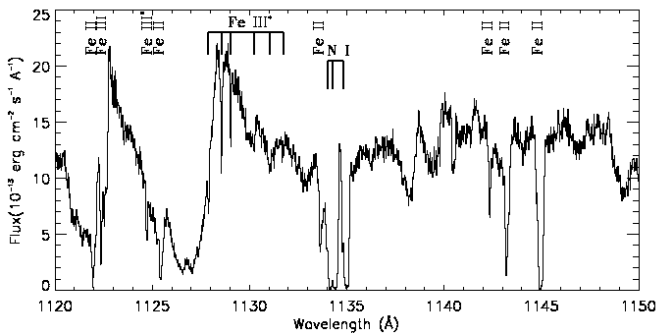
FIG. 1.—Portion of the FUSE LiF 2A spectrum of SwSt 1 from 1120 to 1150 Å. The data have been rebinned by 3 pixels, corresponding to a pixel size of 0.02 Å. Nebular absorption lines (which are much narrower than the broad stellar features) are identified above the spectrum; asterisks denote absorption from excited levels.
