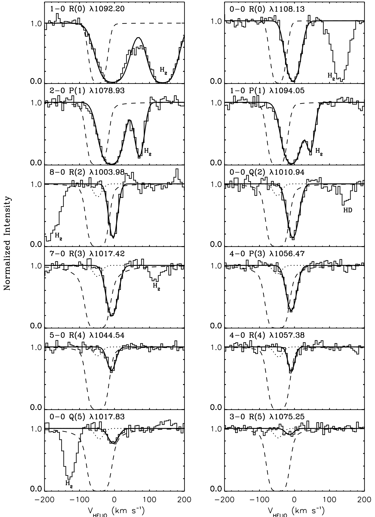
FIG. 3.—Continuum-normalized profiles of selected \text{H}_2 transitions from Table 7 plotted against heliocentric velocity. For comparison, we also display relatively weak (small f -value) lines from the J = 0 and 1 levels, for which no N_J upper limits were measured. Two transitions from each rotational level are shown and are arranged from top to bottom in order of increasing J . All lines are from the Lyman band, with the exception of the Werner lines 0-0 Q(2) \lambda 1010.94 and 0-0 Q(5) \lambda 1017.83 . Absorption from other species is indicated within the panels. Fits to the interstellar component (and blends with nearby lines) are depicted by thick solid lines. The dotted lines represent nebular absorption profiles with column densities equal to the measured upper limits given in Table 7 [if both N(\text{rms}) and N(\text{fit}) are available, we select the smallest of the two]. Dashed lines illustrate the absorption profiles expected if the nebular column density of \text{H}_2 is as high as indicated by the infrared emission lines, assuming T_{\text{rot}} = 1600 K (for lower T_{\text{rot}} , the nebular absorption profiles would be even more deeply saturated, since the emitting v = 1, J = 3 level would have a smaller fractional population).
